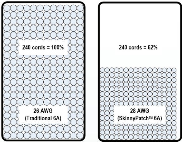
Fill Comparison: Category 6A UTP Cords in a 6 in. x 3.5 in. (152.4 x 89mm) cable manager
